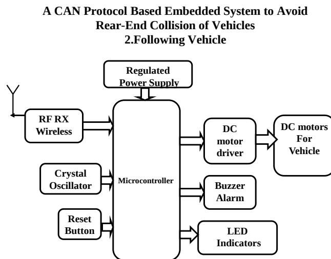
FIG 2: Block diagram of CAN based real time implementation in automobile
